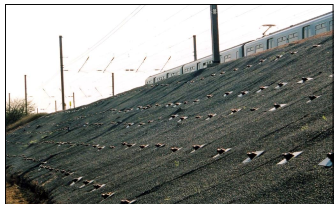
MacMat® R and soil nail reinforced slope
